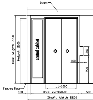
Entrance plan Top Floor
