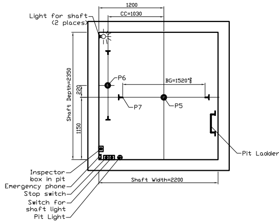
Lift Plan (for installation reference)
