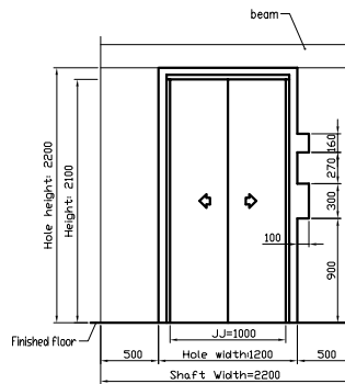
Entrance plan Main Floor
