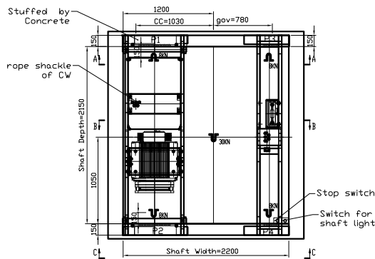
Top Beam Layout (for installation reference)
