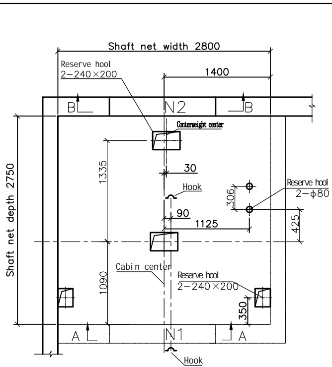
Machine room reserved hook plane drawing
