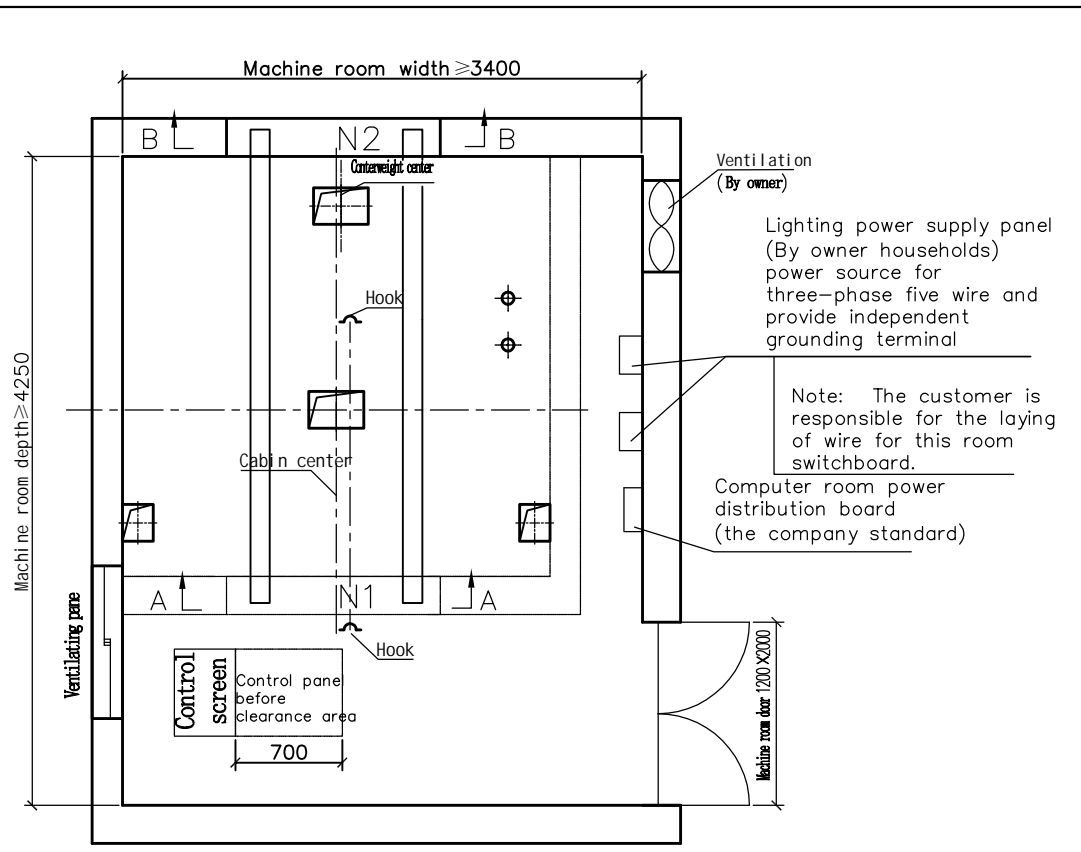
Machine room plane layout
